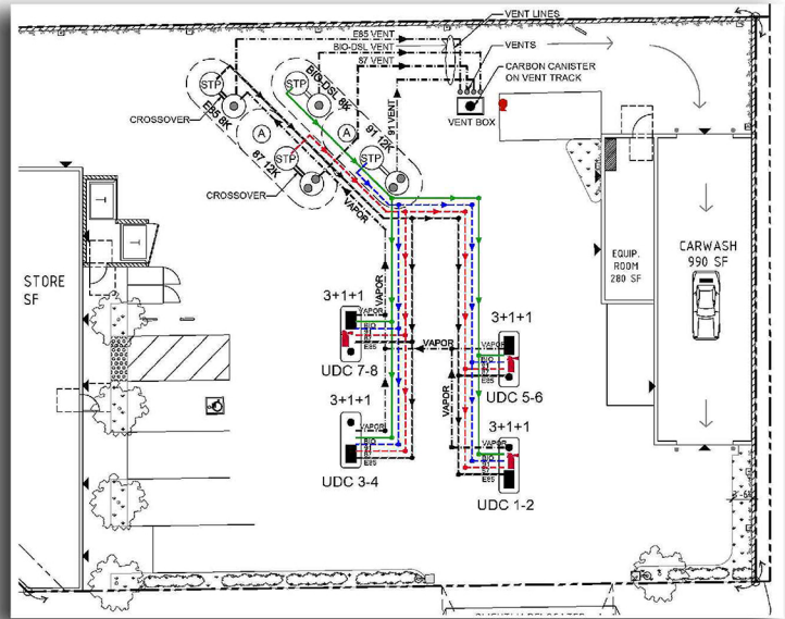
• PLAN OF FUELING SYSTEM
